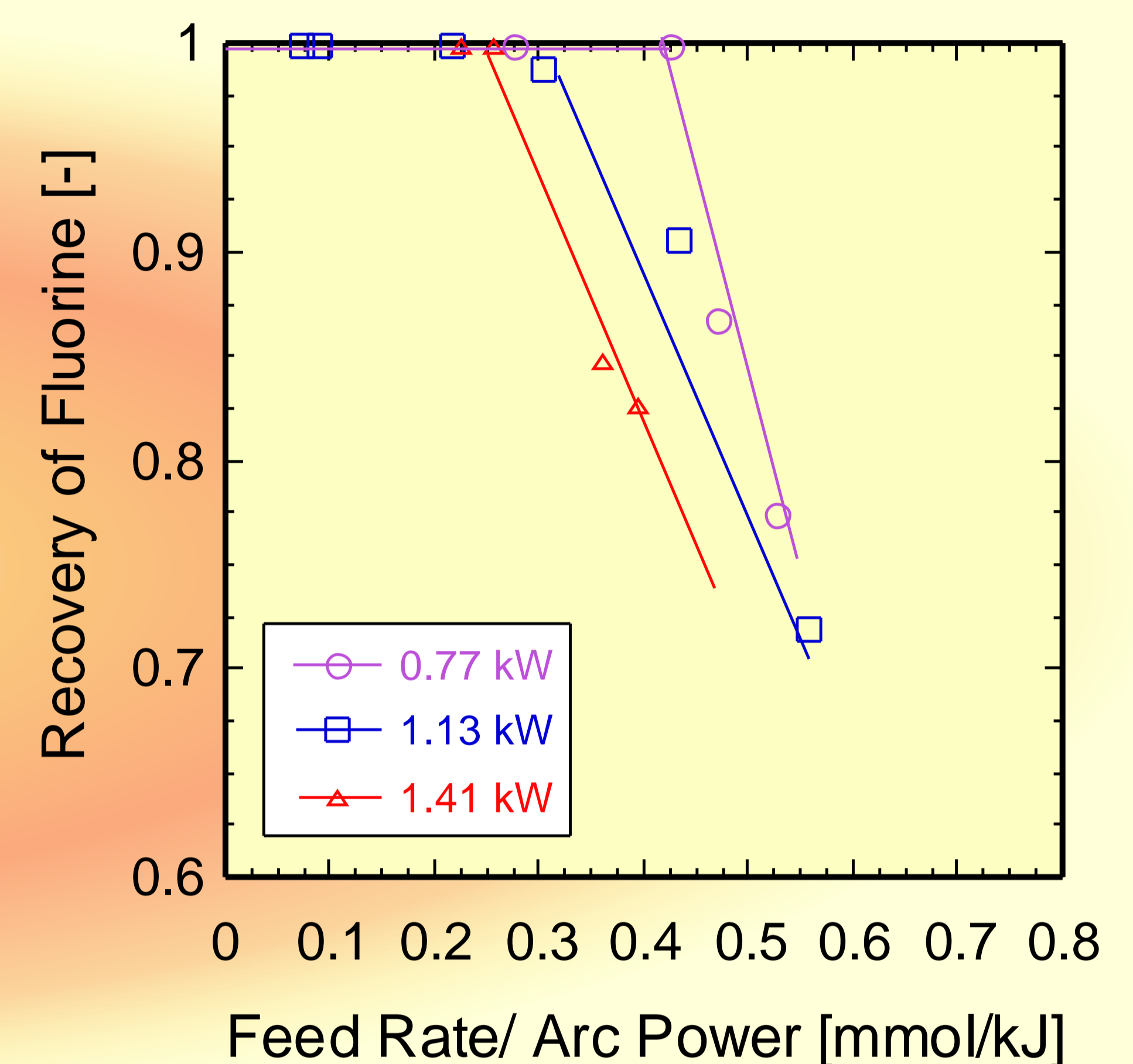
Fluorine recovery (indicating HFC destruction)
